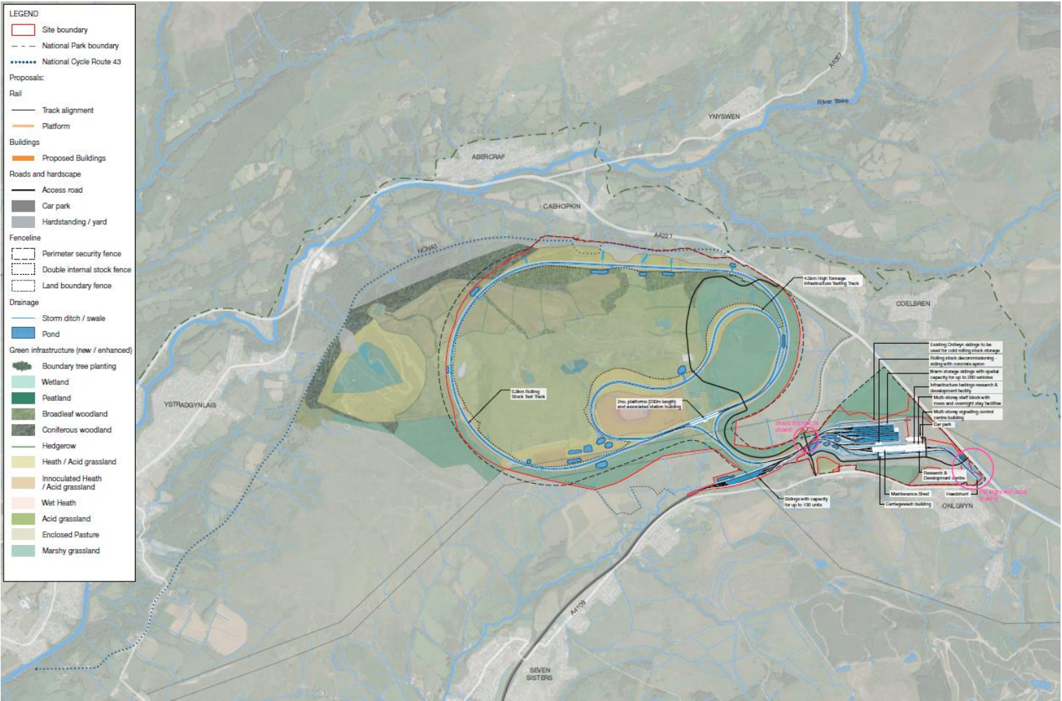
Figure 17: Proposed site layout (preliminary)
