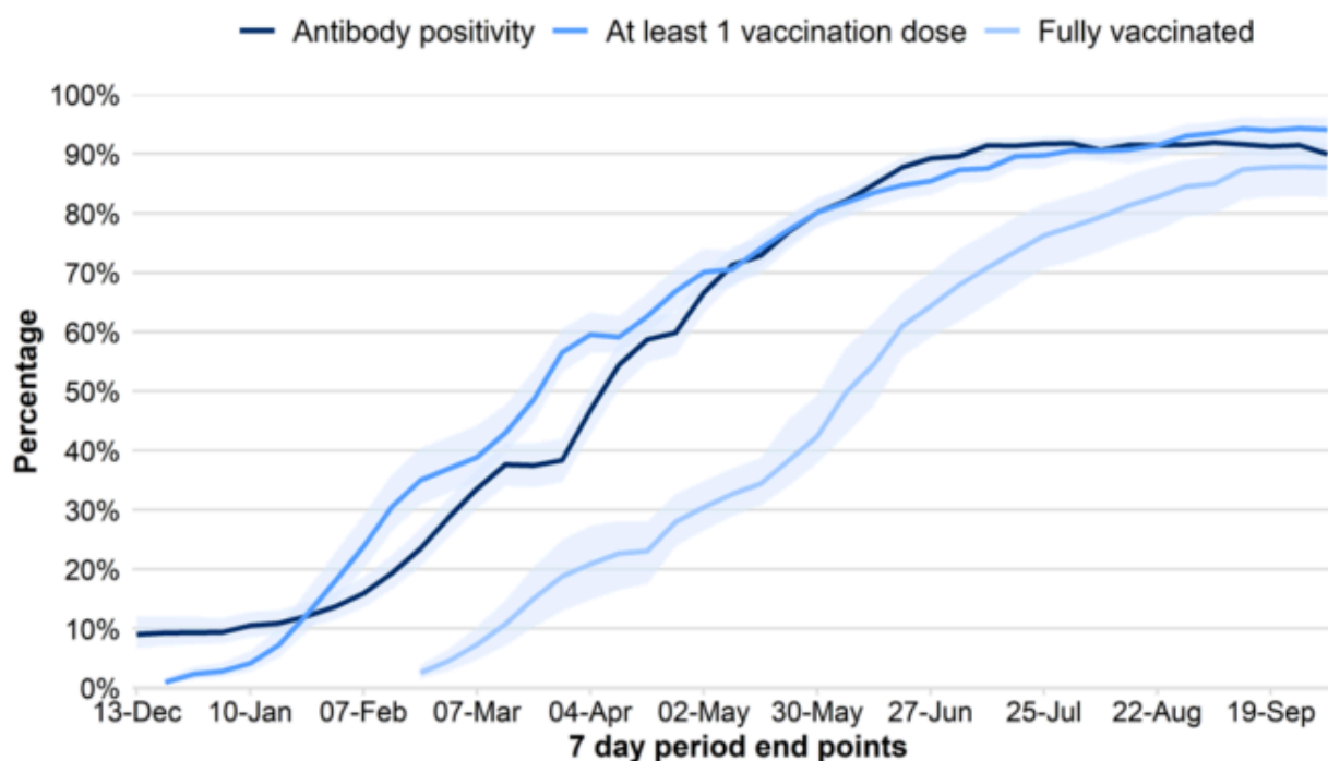
Chart 2: Estimated percentage of the population in Wales reporting receipt of vaccination and testing positive for coronavirus (COVID-19) antibodies from 7 December 2020 to 3 October 2021
