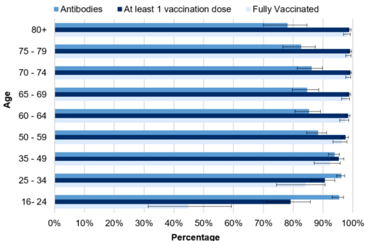
Chart 3: Estimated percentage of the population in Wales reporting receipt of vaccination and testing positive for coronavirus (COVID-19) antibodies by age group, 27 September to 3 October 2021
