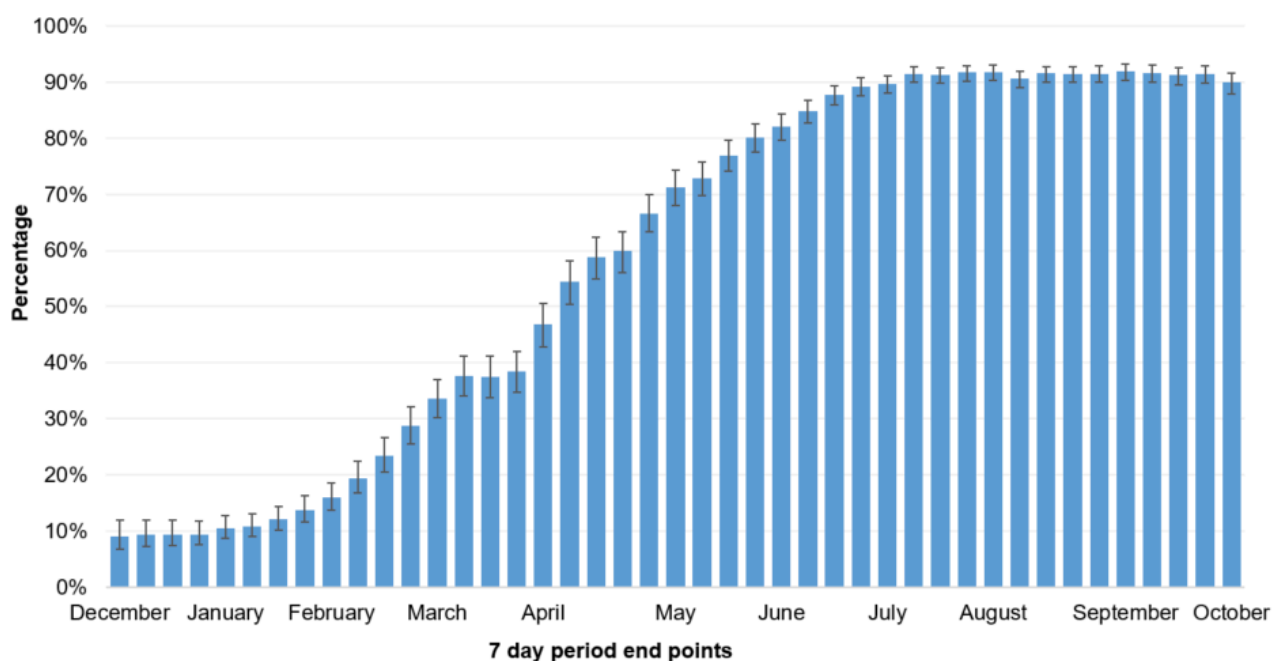
Chart 1: Estimated percentage of the population in Wales testing positive for coronavirus (COVID-19) antibodies, December 2020 to October 2021
