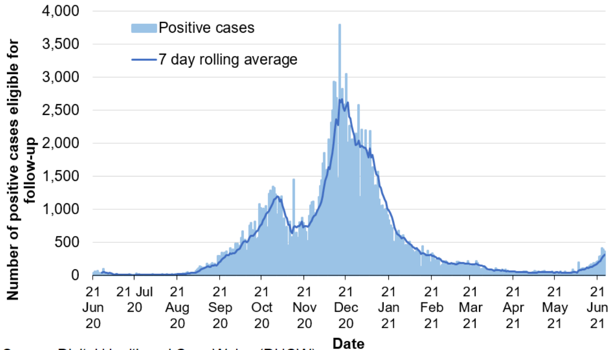
Chart 3: Daily positive cases eligible for follow-up by local contact tracing teams, up to 26 June 2021
