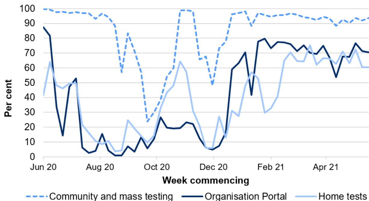
Chart 5: Proportion of antigen tests authorised in one calendar day through non-NHS Wales laboratories as at end 13 June 2021
