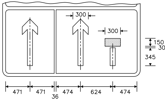
2 lane carriageway plus hard shoulder
