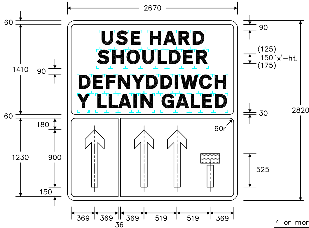
3 lane carriageway plus hard shoulder
