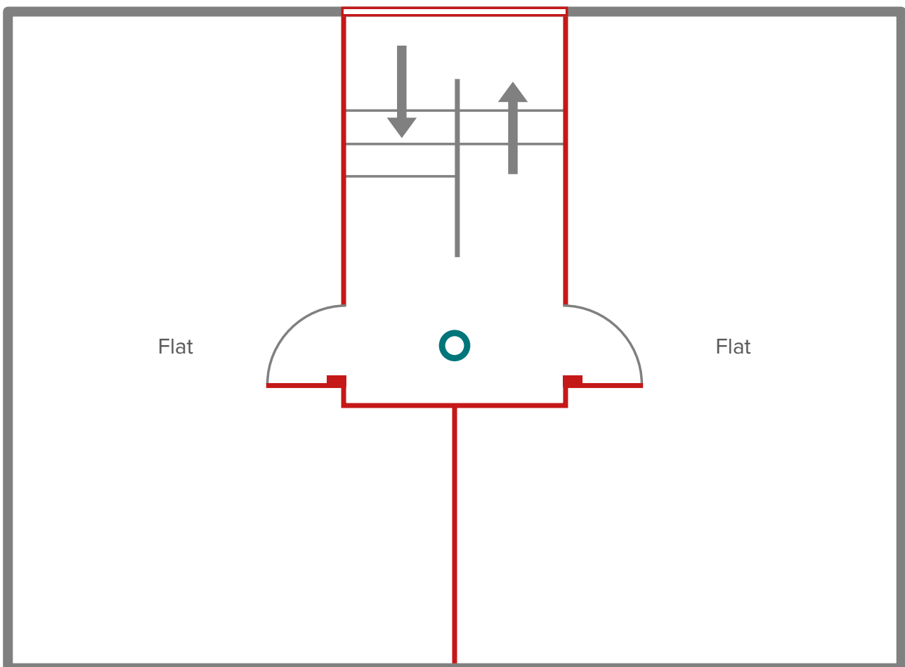
Figure 7 – Flats opening directly onto a stairway
