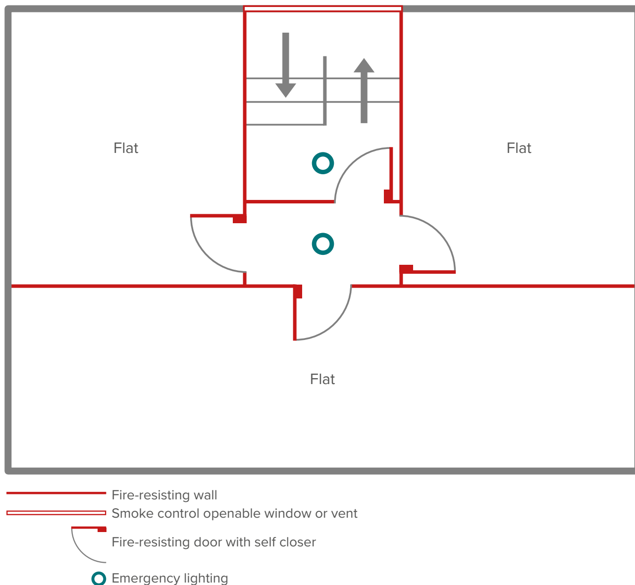
Figure 8 – Lobby access to flats onto stairs
