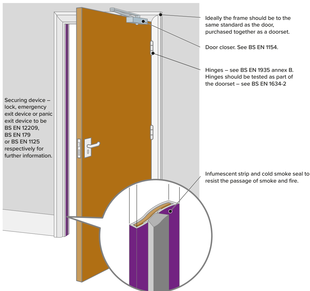
Figure 9 – A modern fire-resisting and smoke stopping door
