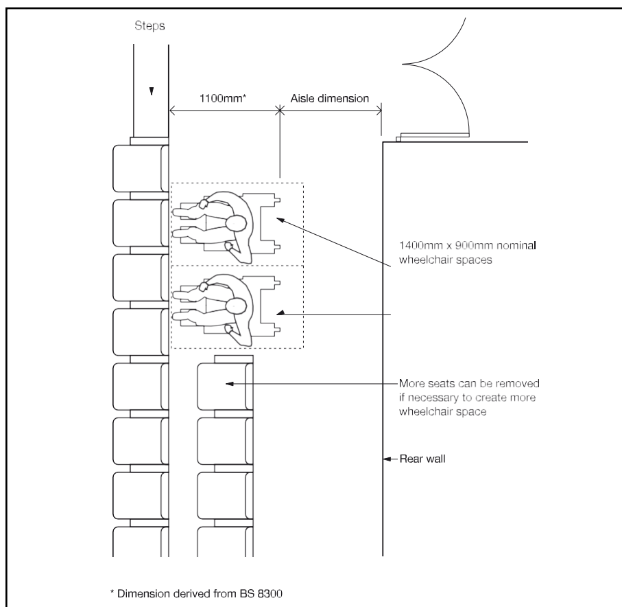
Diagram 14 Possible location of wheelchair spaces in front of a rear aisle
