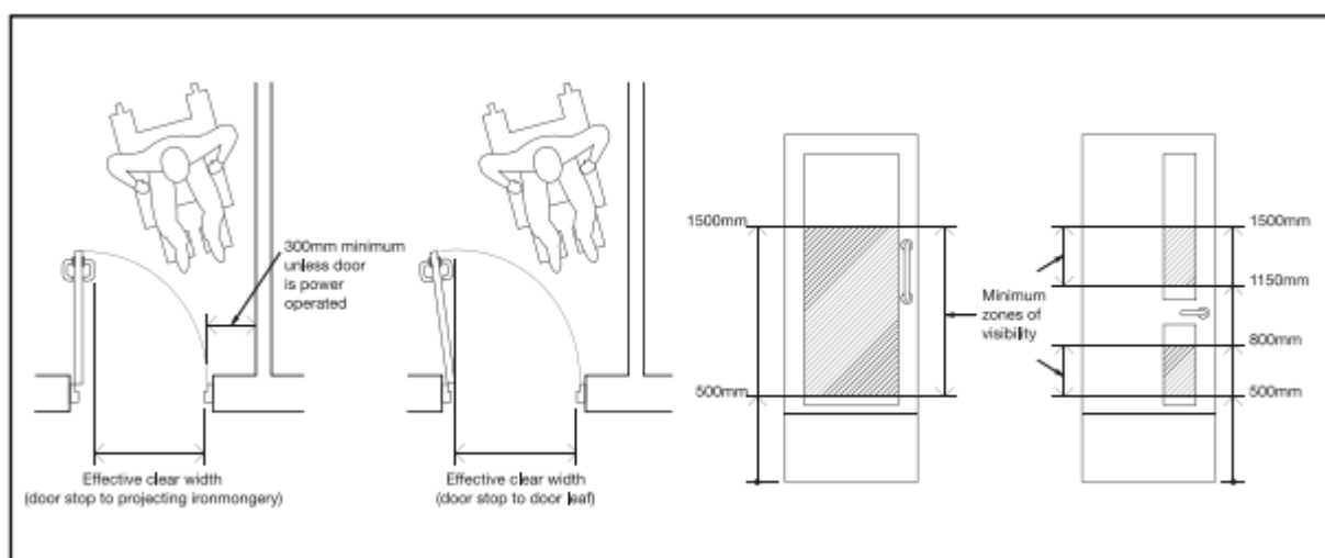
Diagram 9 Effective clear width and visibility requirements of doors
