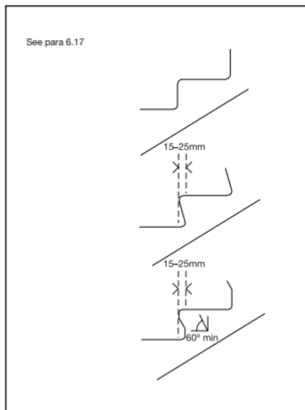
Diagram 27 External step profiles
