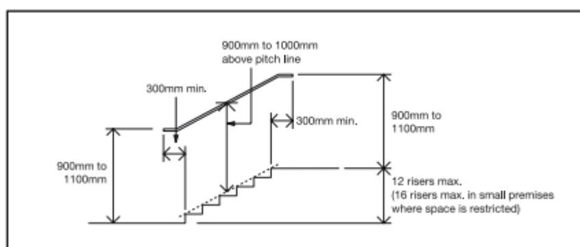
Diagram 12 Internal stairs – key dimensions
