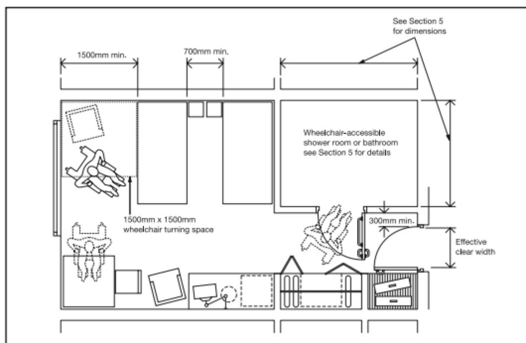
Diagram 17 One example of a wheelchair-accessible hotel bedroom with en-suite sanitary facilities
