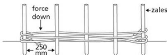
Waffle fence / hurdles
