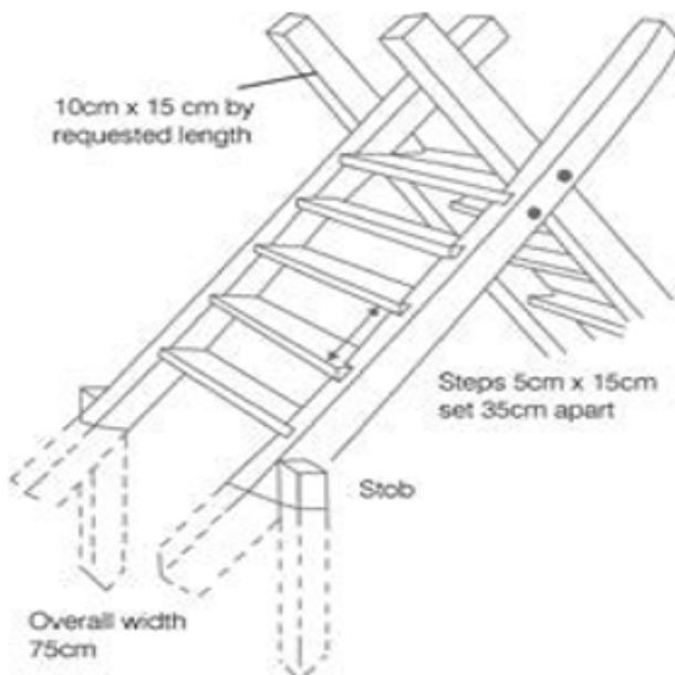
Example of a step ladder stile
