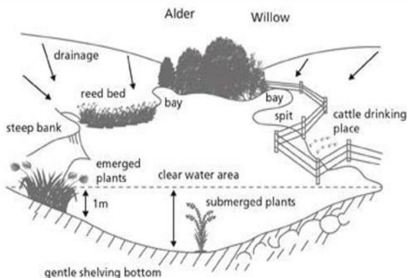
Diagram – Cross Section of Pond
