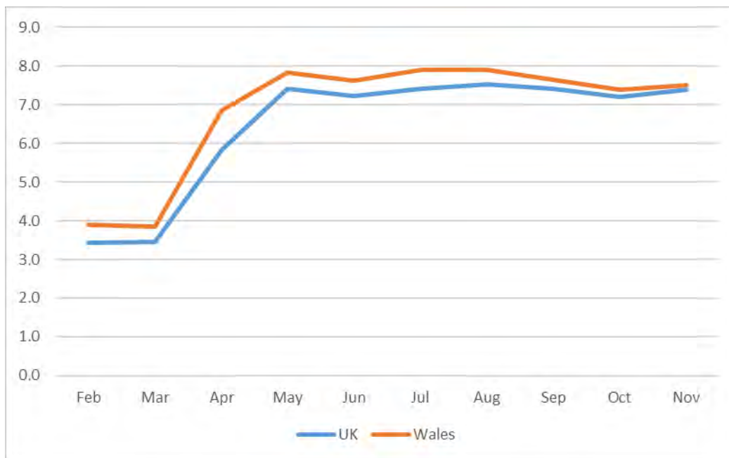
Chart 3: Claimant Count
