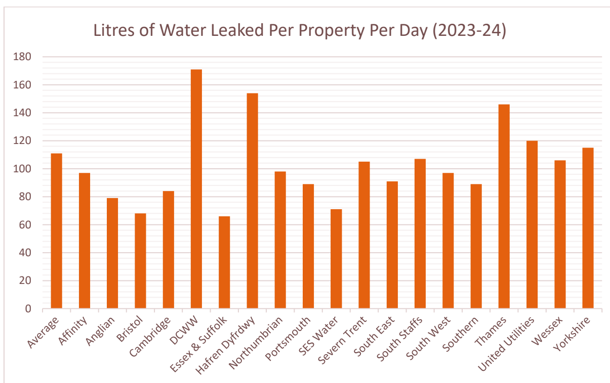
Figure 4.1 - Water leakage rates per Property by Water Company (this graph shows the average leakage per property per day for the latest three years compared to the number of properties in the latest year). Source: Discover Water 39
