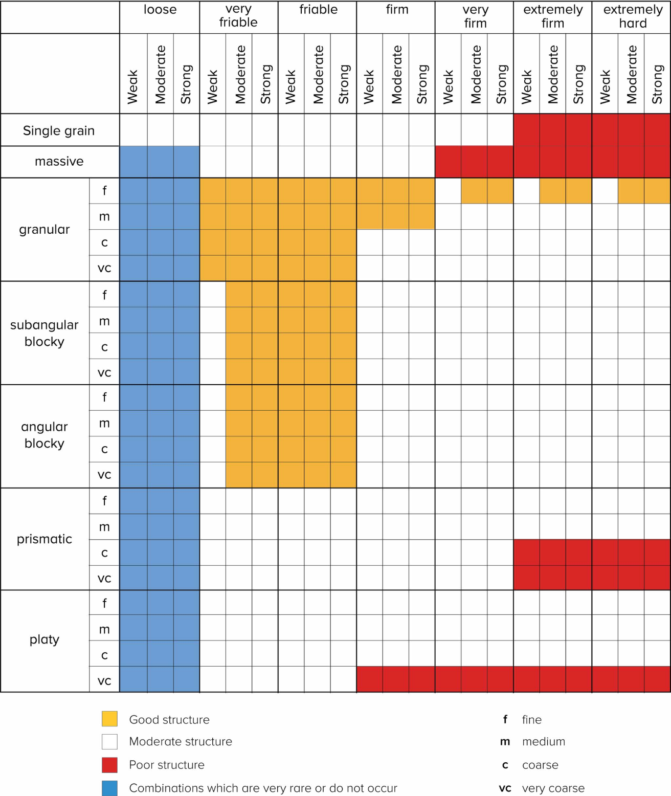
Figure 9: Assessment of structural conditions 1 in subsoil horizons with S or LS texture
