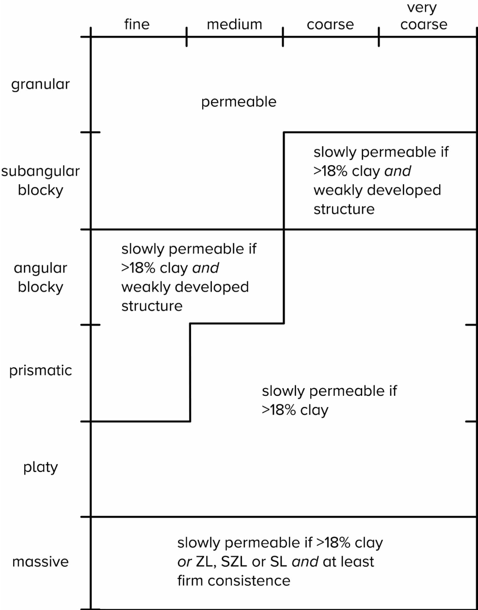
Figure 5: Diagrammatic representation of the combinations of structure, texture and consistence which are characteristic of slowly permeable layers
